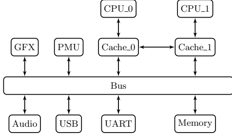
Figure 1: The block diagram of the simple SoC model.
